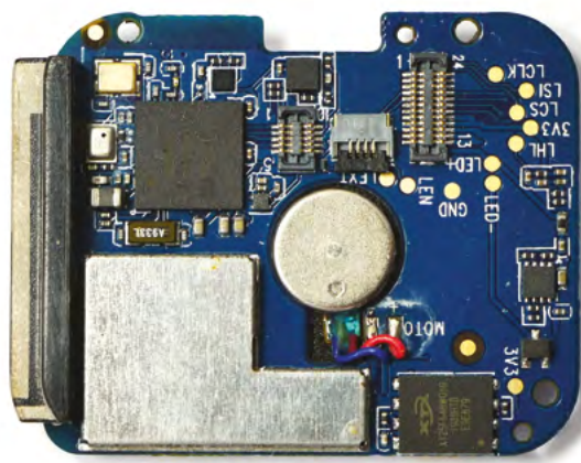
▲ The PCB inside Bangle.js 2
