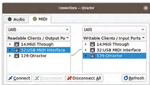
▲ Qtractor uses JACK's MIDI connector to direct output from the DAW to your USB MIDI interface
