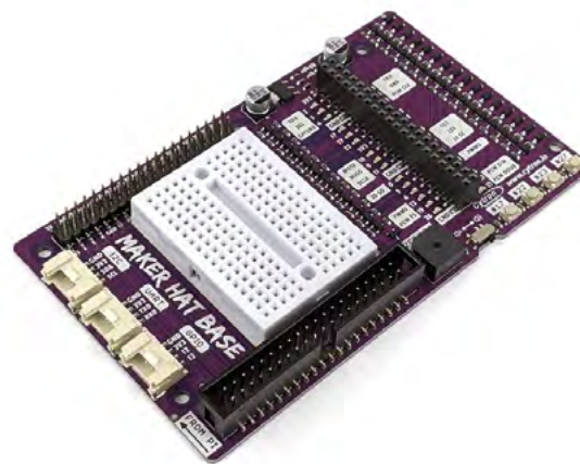
▲ The board also acts as a mini electronics lab, complete with breadboard, buzzer, buttons, and breakout header
